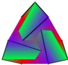
A planar unfolding of the Boy Surface
